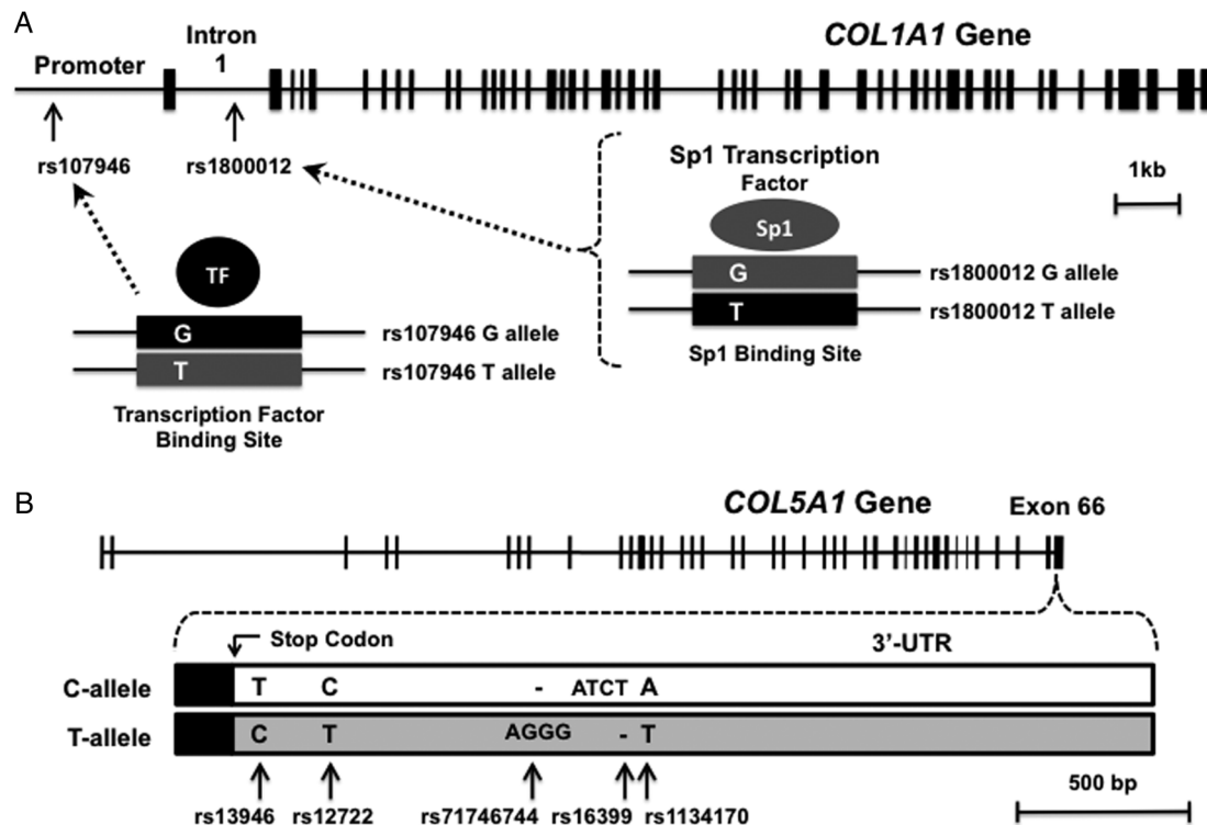
Figure 2 A schematic representation of the exon (vertical lines) and intron (horizontal lines) boundaries of the human (A) COL1A1 and (B) COL5A1 genes. The functional variants within the promoter region (rs107946, G/T) and first intron (rs1800012, G/T) of COL1A1 are indicated. Both these variants are located in transcription factor binding sites, namely an unknown transcription factor binding site in the promoter and an Sp1 binding site in intron 1, which have been expanded. The variant within each binding site affects the affinity of the binding of the respective transcription factor. Increased binding and transcription have been reported to the alleles in black (ie, G allele of rs107946 and the T allele of rs1800012). An increased \alpha 1(I) chain is produced from these alleles. Two forms of COL5A1 exon 66, which encodes for the terminal amino acids of the \alpha 1(V) chain (black box), the stop codon and the 3'-untranslated region (UTR) (clear and grey boxes), are indicated. The four variants, rs13946 (C/T), rs12722 (C/T), rs71746744 (-/AGGG), rs16399 (ATCT/-) and rs1134170 (A/T), reported to be associated with musculoskeletal soft tissue injuries, are indicated. The variants in the 3'-UTR indicated in grey are generally associated with musculoskeletal soft tissue injuries and determine one of the two major functional forms of the 3'-UTR (T allele) which has been reported to have increased mRNA stability. All the information used to construct this figure was obtained from Ensembl ( http://www.ensembl.org ).
