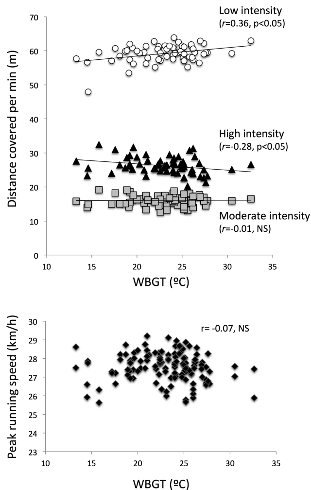
Figure 2 Upper part: distance covered at low (speed <11 km/h), moderate (speed 11–14 km/h) and high (speed >14 km/h) intensity during the 2014 FIFA World Cup matches in relation to WBGT. Lower part: peak running speed as a function of WBGT during the 2014 World Cup matches (NS, not significant; WBGT, wet-bulb globe temperature).
